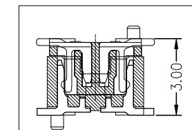
ASSEMBLY
