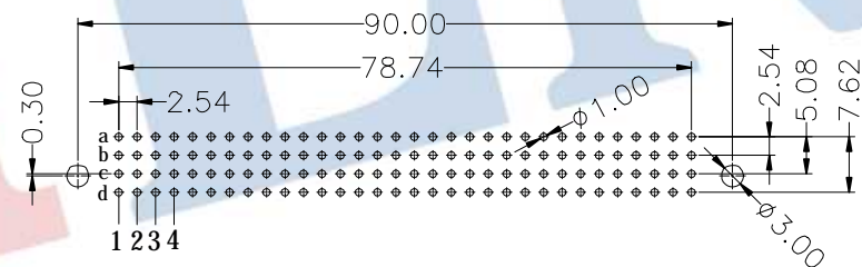
Recommended P.C.B Layout(Top Side) (PCB BOARD TOLERANCE±0.05)
