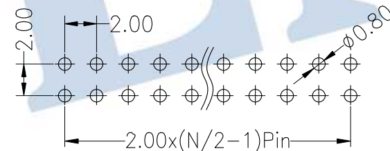
Recommended P.C.B Layout(Top Side) (PCB BOARD TOLERANCE±0.05)
